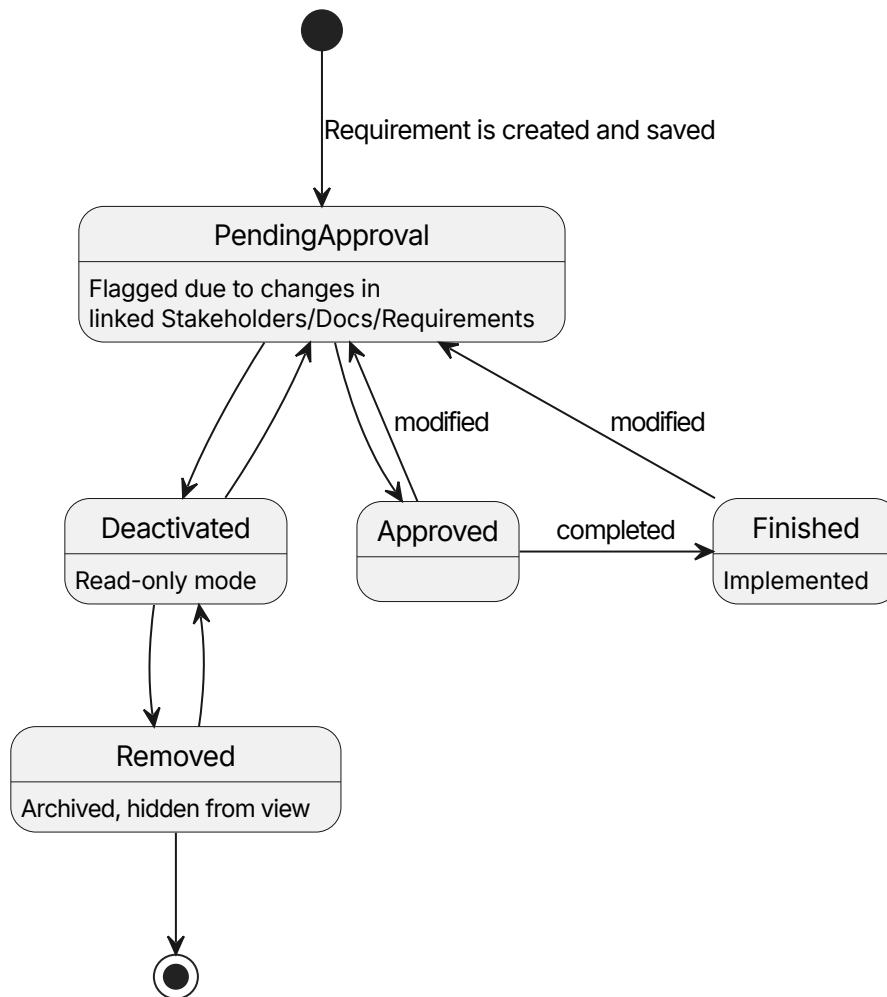
Figure 2: Requirement entity's state diagram
