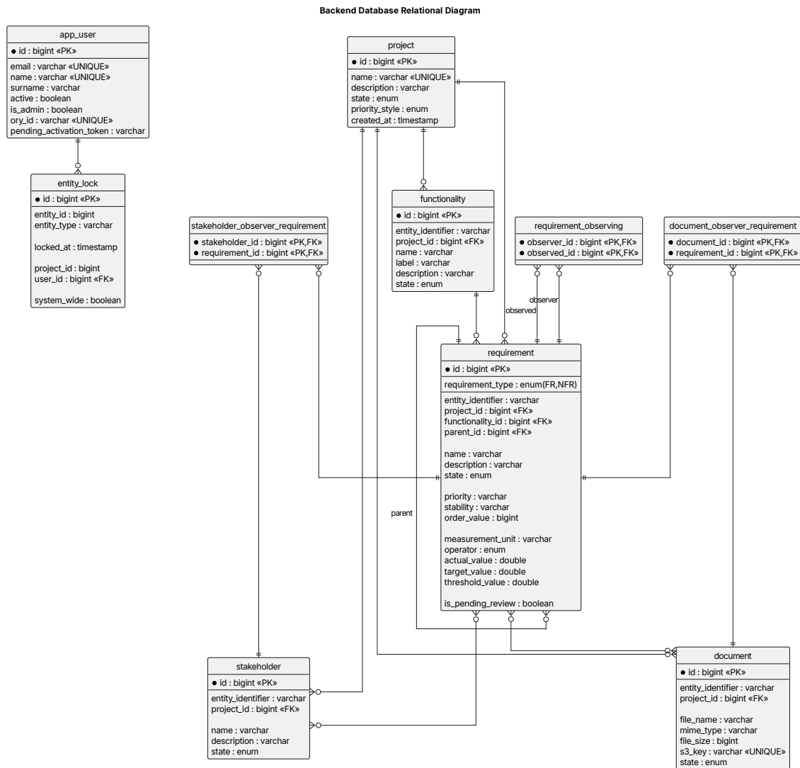
Figure 14: Relational database schema
