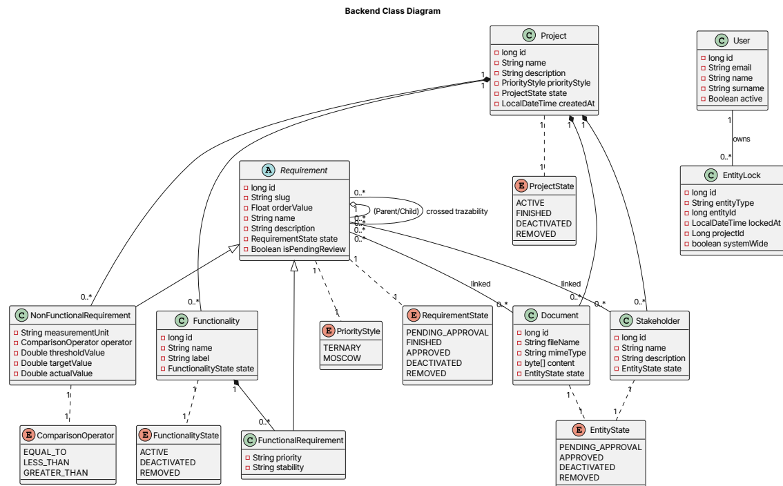
Figure 13: Domain class diagram
