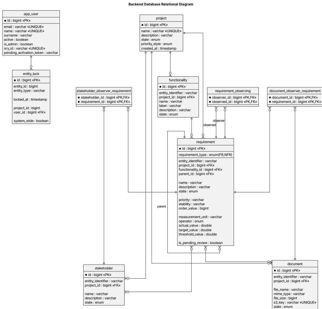
Figure 24: Relational database schema
