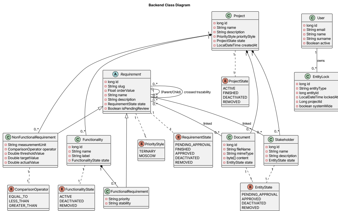
Figure 23: Domain class diagram
