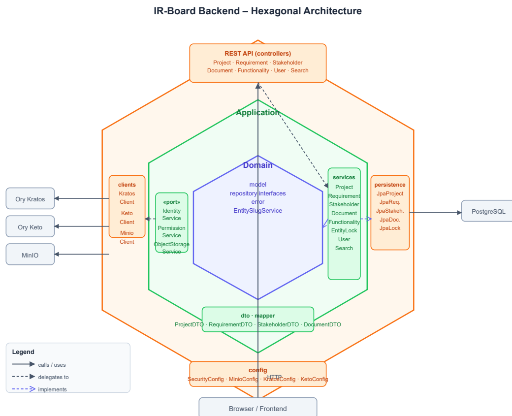
Figure 22: Backend hexagonal architecture diagram
