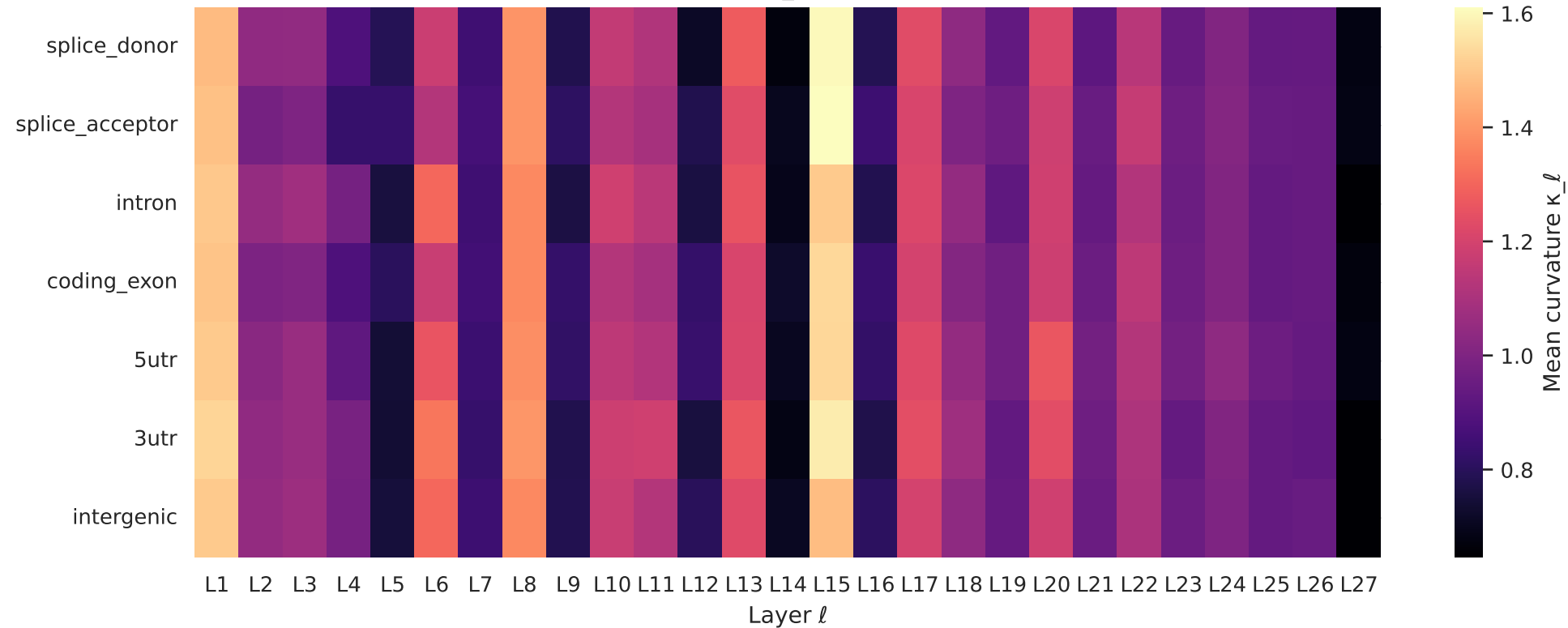
V3 (zoom L1-27) curvature \kappa_\ell — clearer per-layer pattern
