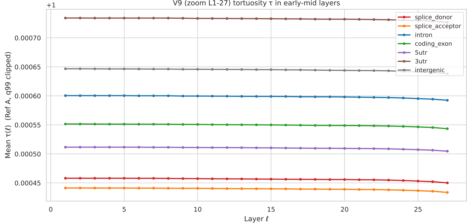
V9 (zoom L1-27) tortuosity \tau in early-mid layers
