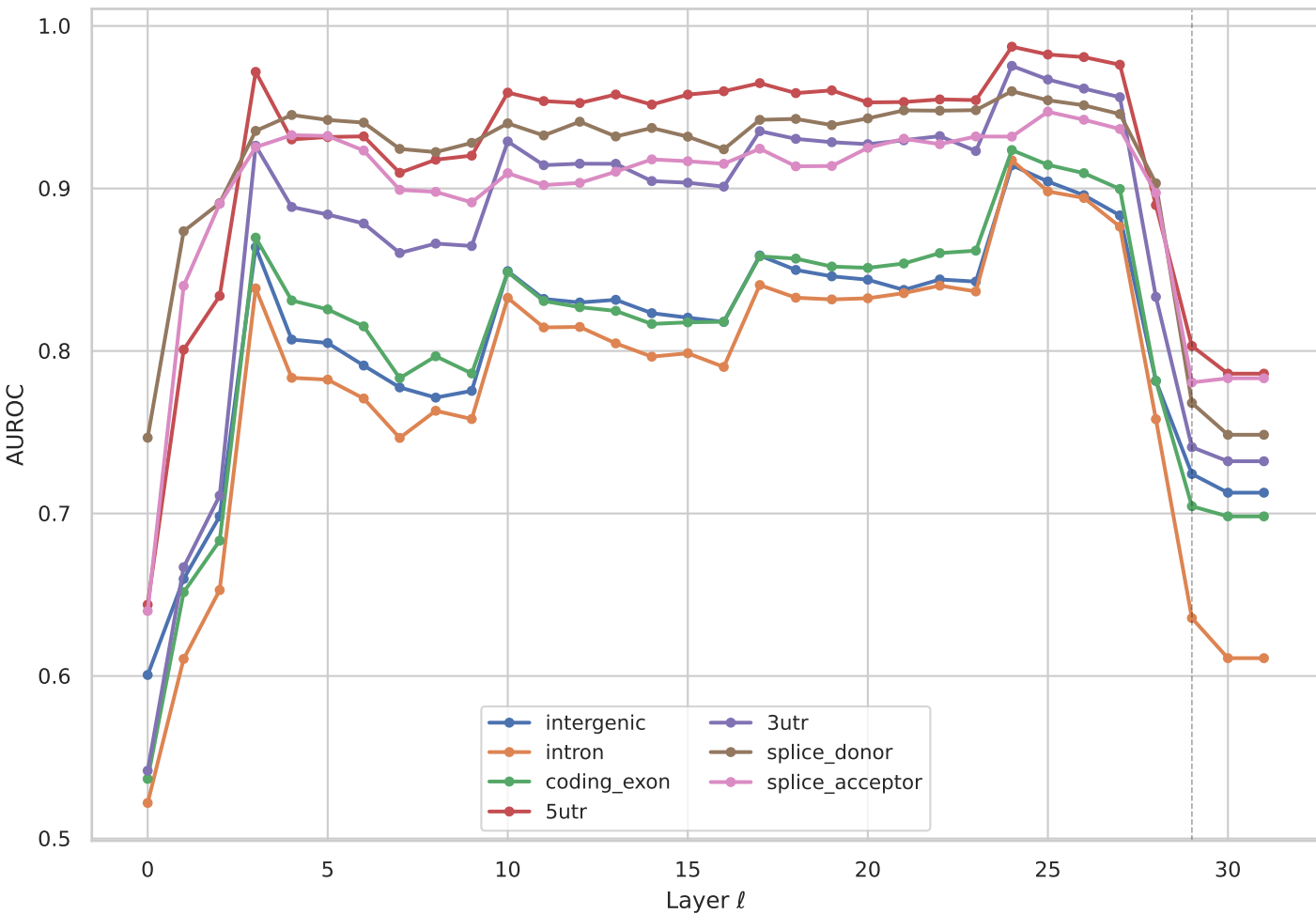
(H4) Per-layer per-class AUROC (OVR)
