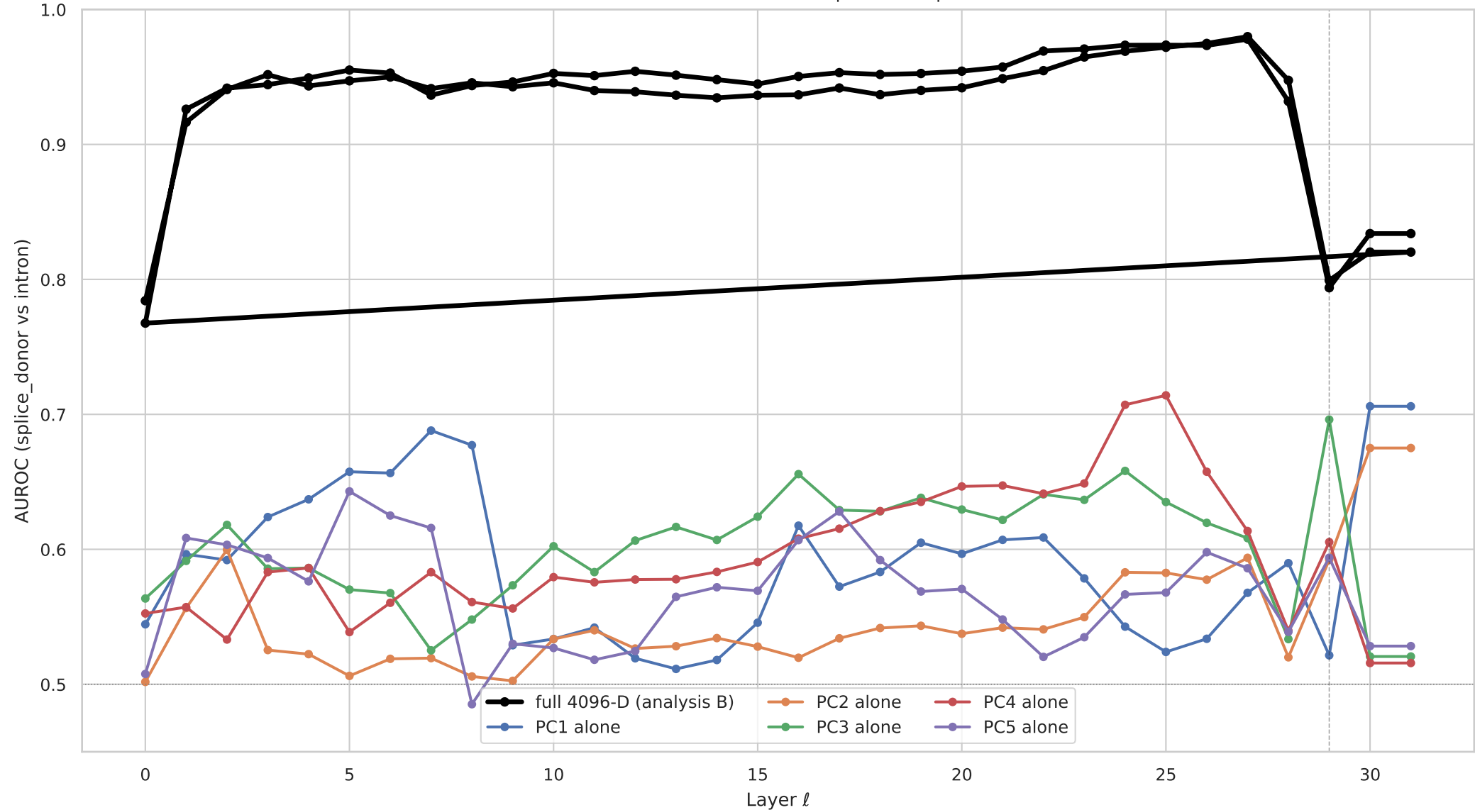
(T1) PC-alone probing AUROC vs full 4096-D probing PC1 close to full = PC1 IS the context axis. Gap = PC1 captures other variance.
