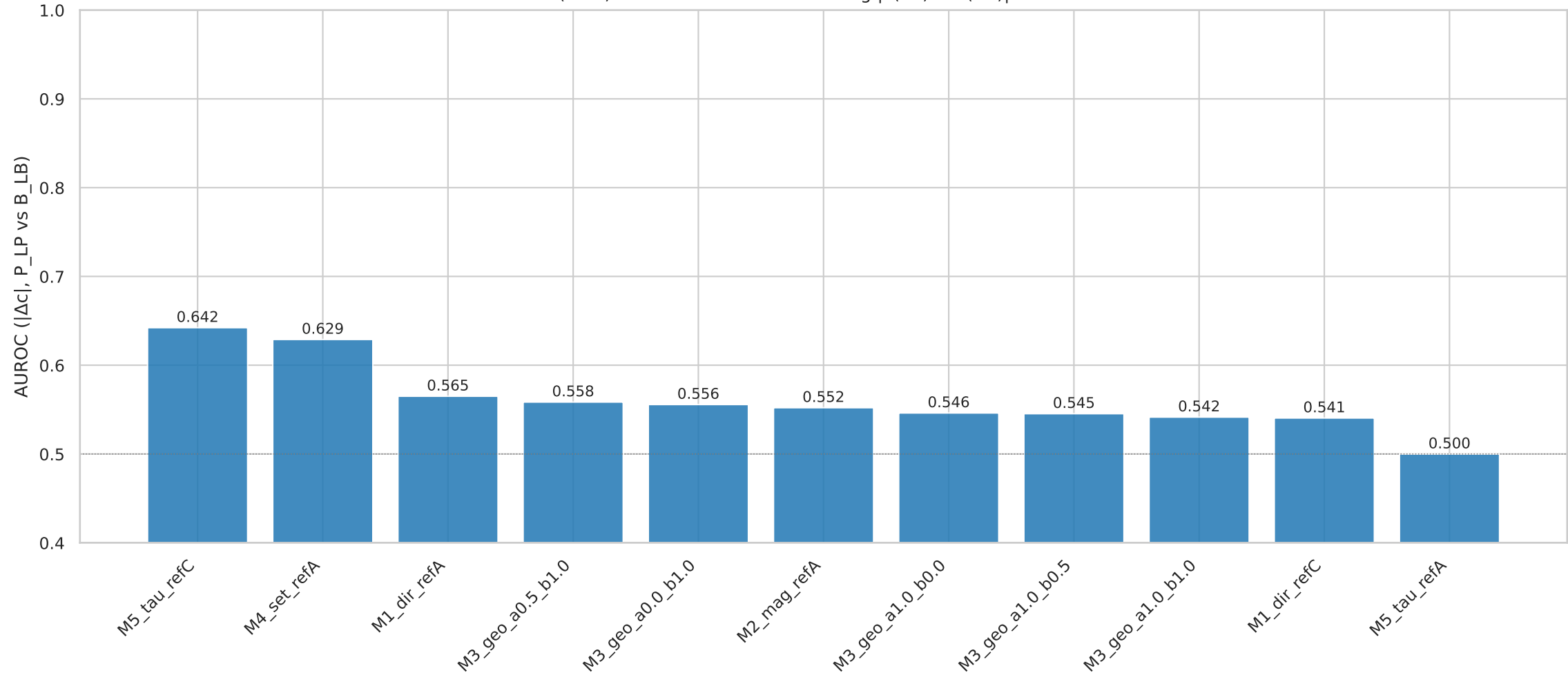
(1.1b) Per-cell variant AUROC using |c(\text{alt}) - c(\text{ref})| as score
