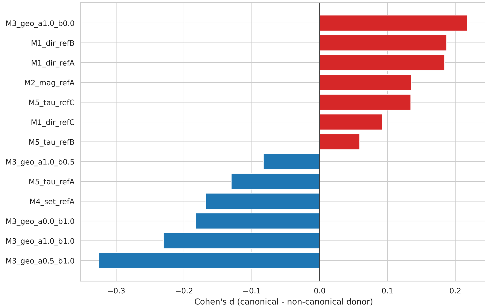
Per-cell discrimination: canonical GT-AG donor (193K) vs non-canonical (5,808)
