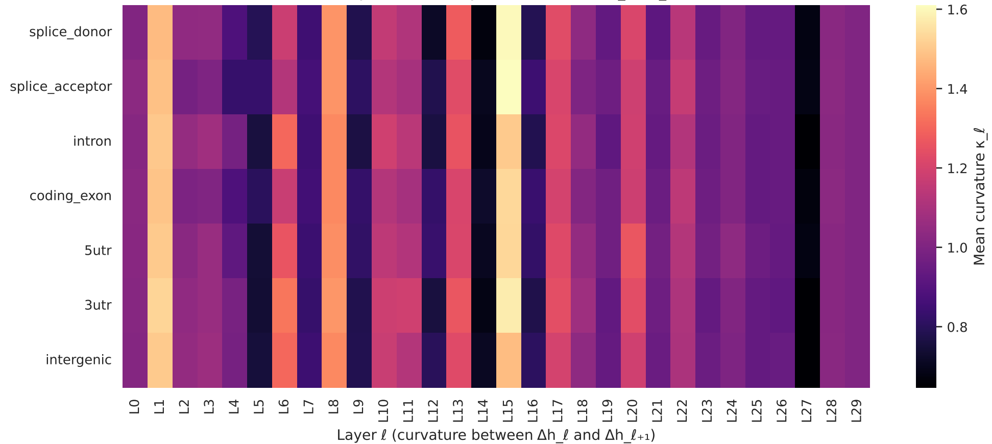
V3 Per-layer curvature by context (1 - \cos(\Delta h_\ell, \Delta h_{\ell+1}) )
