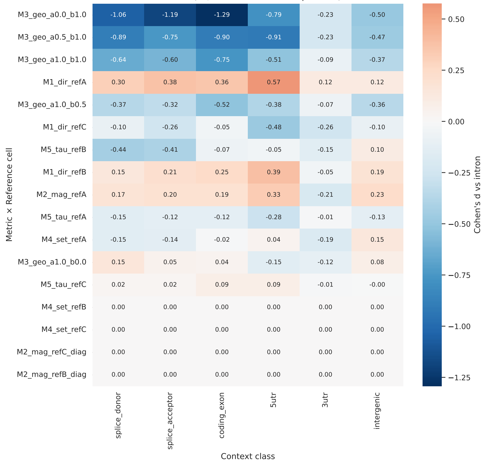
Per-cell × per-context Cohen's d vs intron baseline chr22 v2 (12,978 windows × 77.9M positions)
