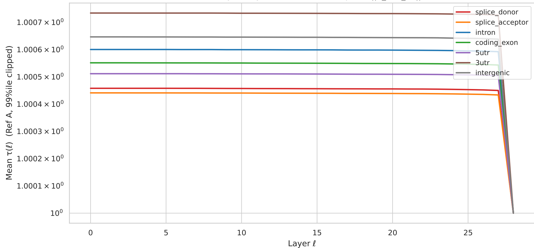
V9 Tortuosity \tau(\ell) by context (Ref A: raw path / ||h_\ell - h_{29}|| )
