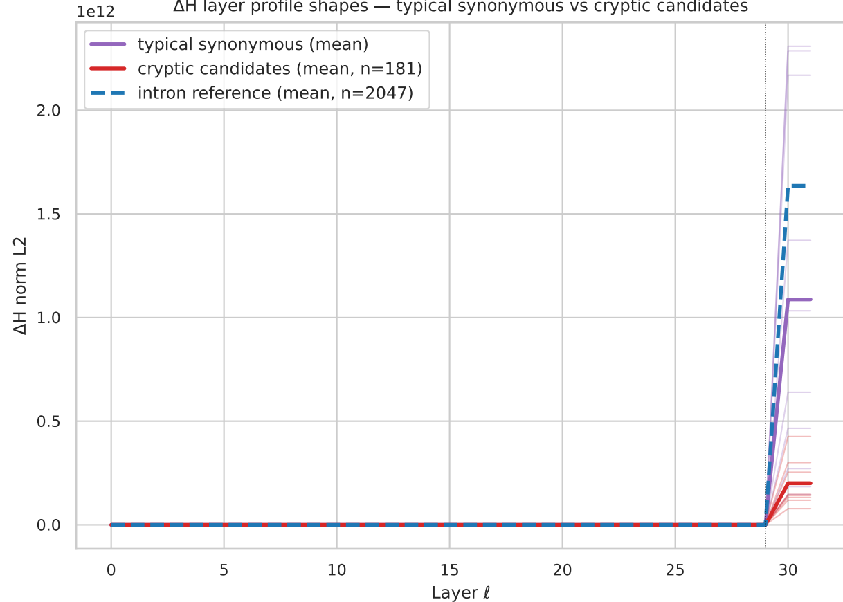
\Delta H layer profile shapes — typical synonymous vs cryptic candidates
