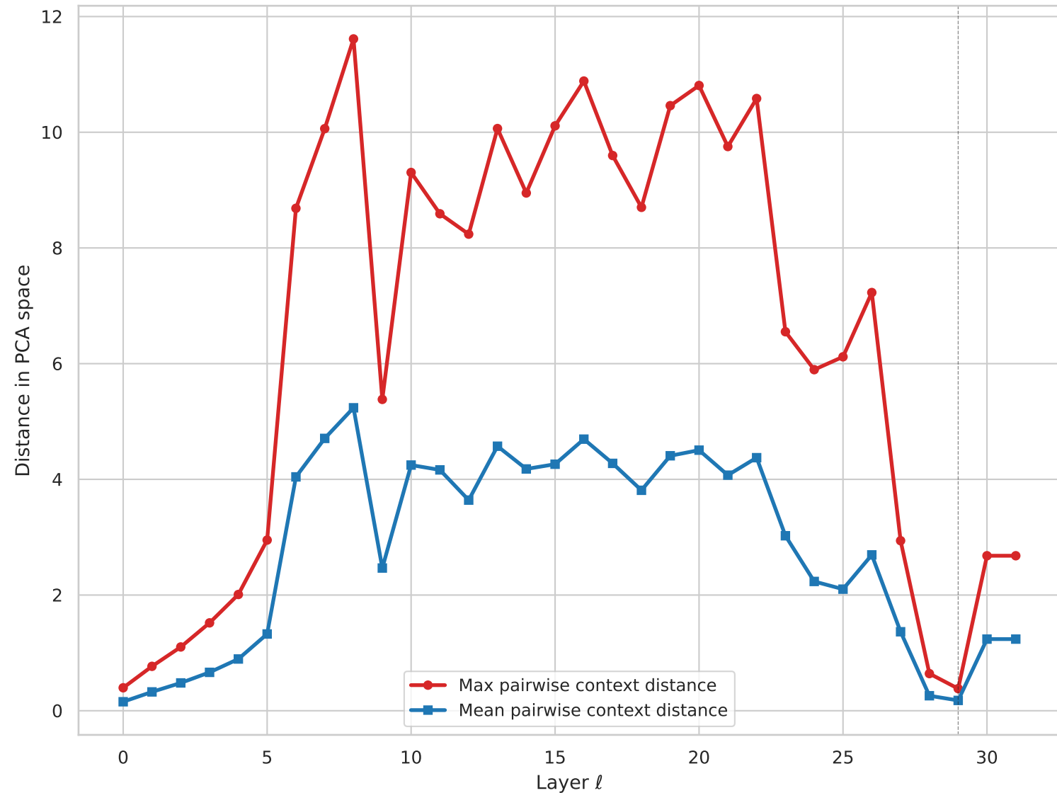
(b2) Context separability per layer Higher = more distinct context representations
