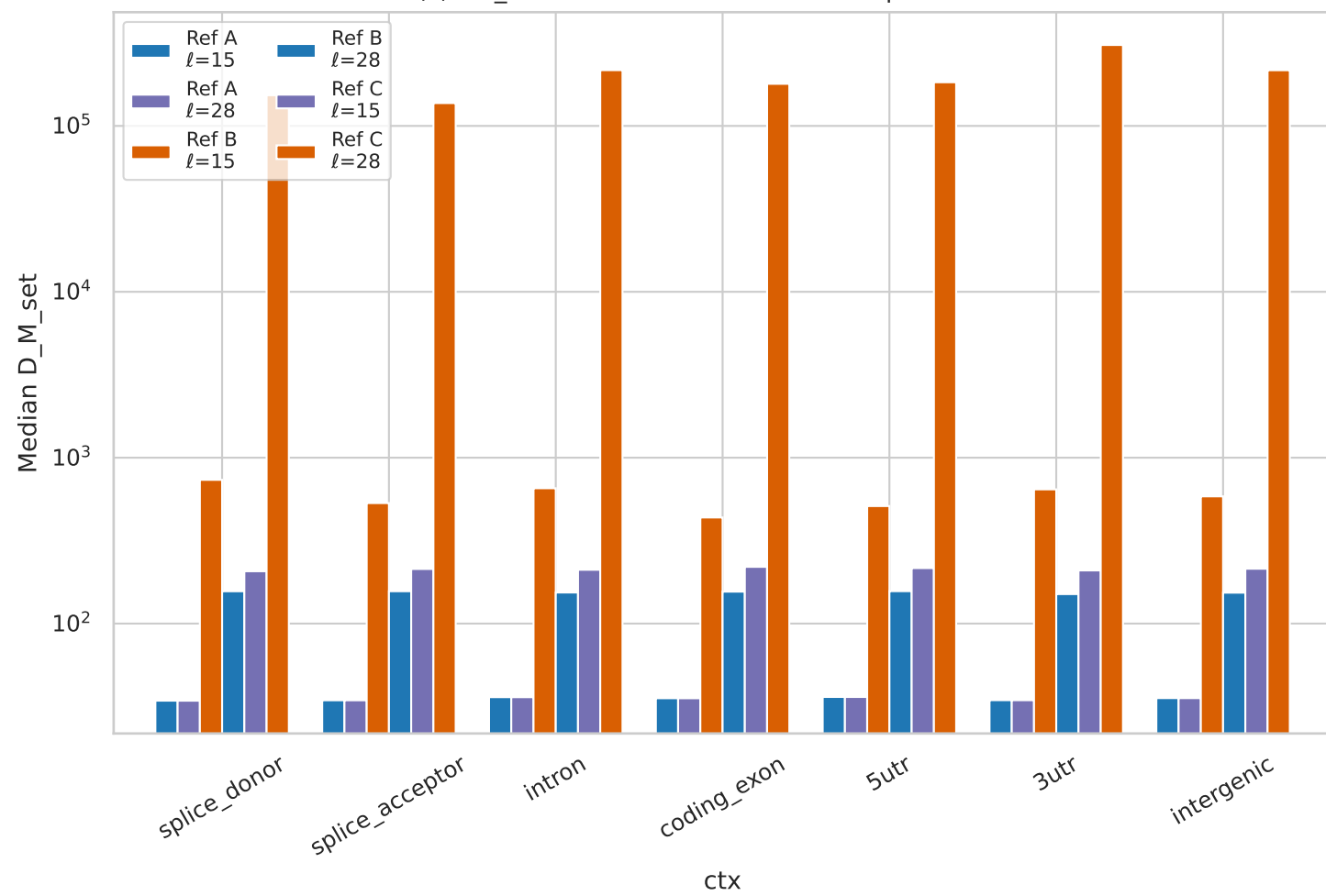
(c) M4_set Ref A/B/C at \ell=15 vs \ell=28 per context
