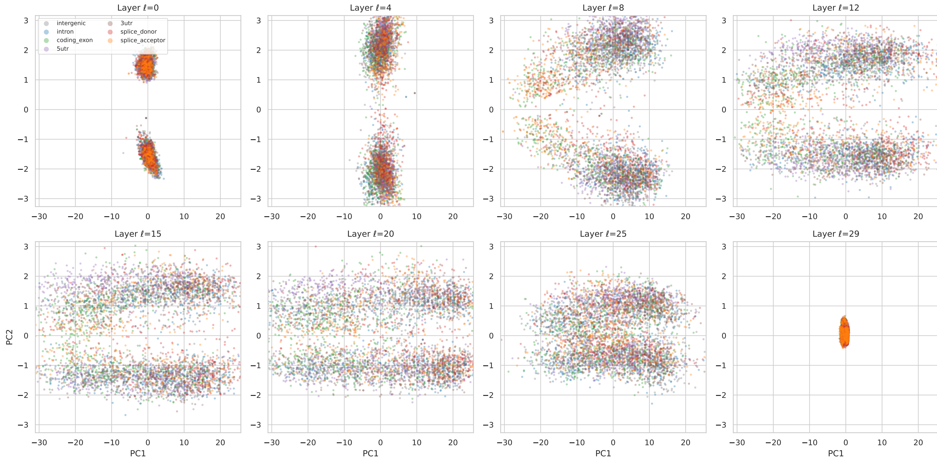
(d) Per-layer PCA snapshots — clusters separate as \ell increases (consistent axes; subsampled 800 tokens/context for plotting)
