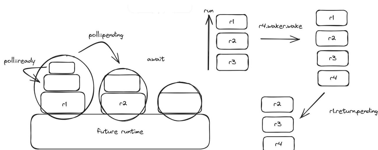
图3-1: NighthawkOS的switch- no- stack
