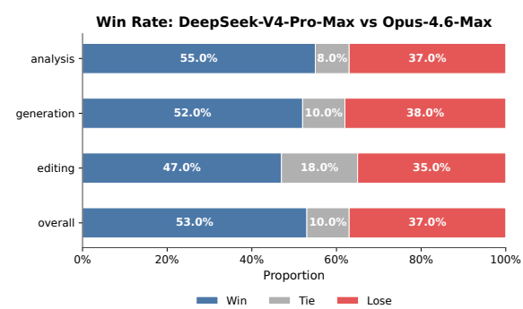
Figure 11 | Win-rate comparison across analysis, generation, editing tasks, and the overall performance.
