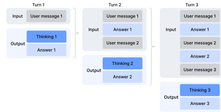
b) Thinking without tools
