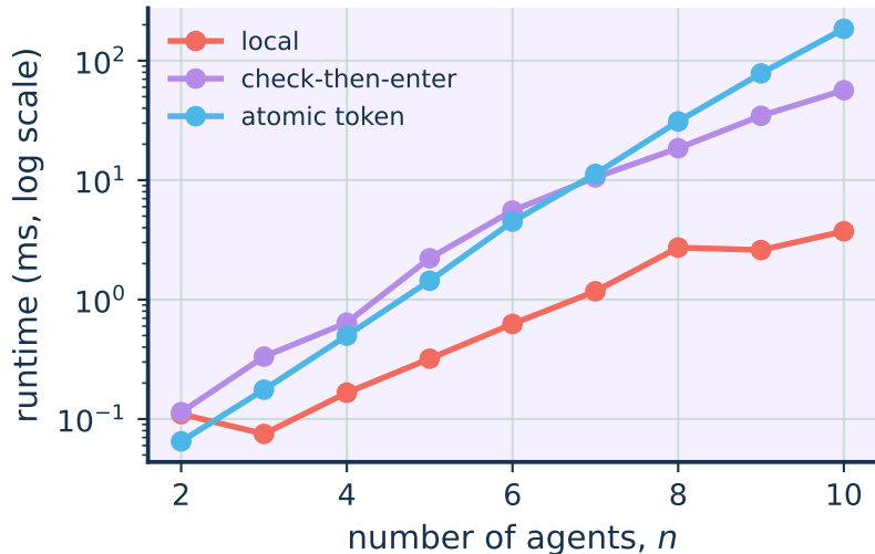
BFS runtime
