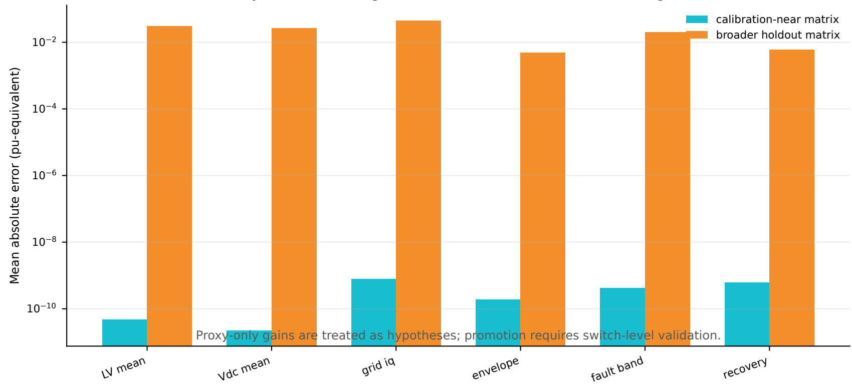
Proxy-to-Simulink alignment: local fit versus holdout ranking risk
