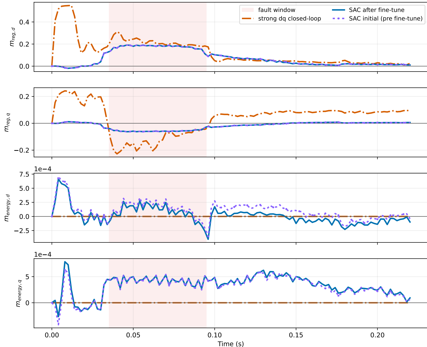
Controller modulation commands per 2-ms control step SAC initial is nearly overlapped by SAC after fine-tune
