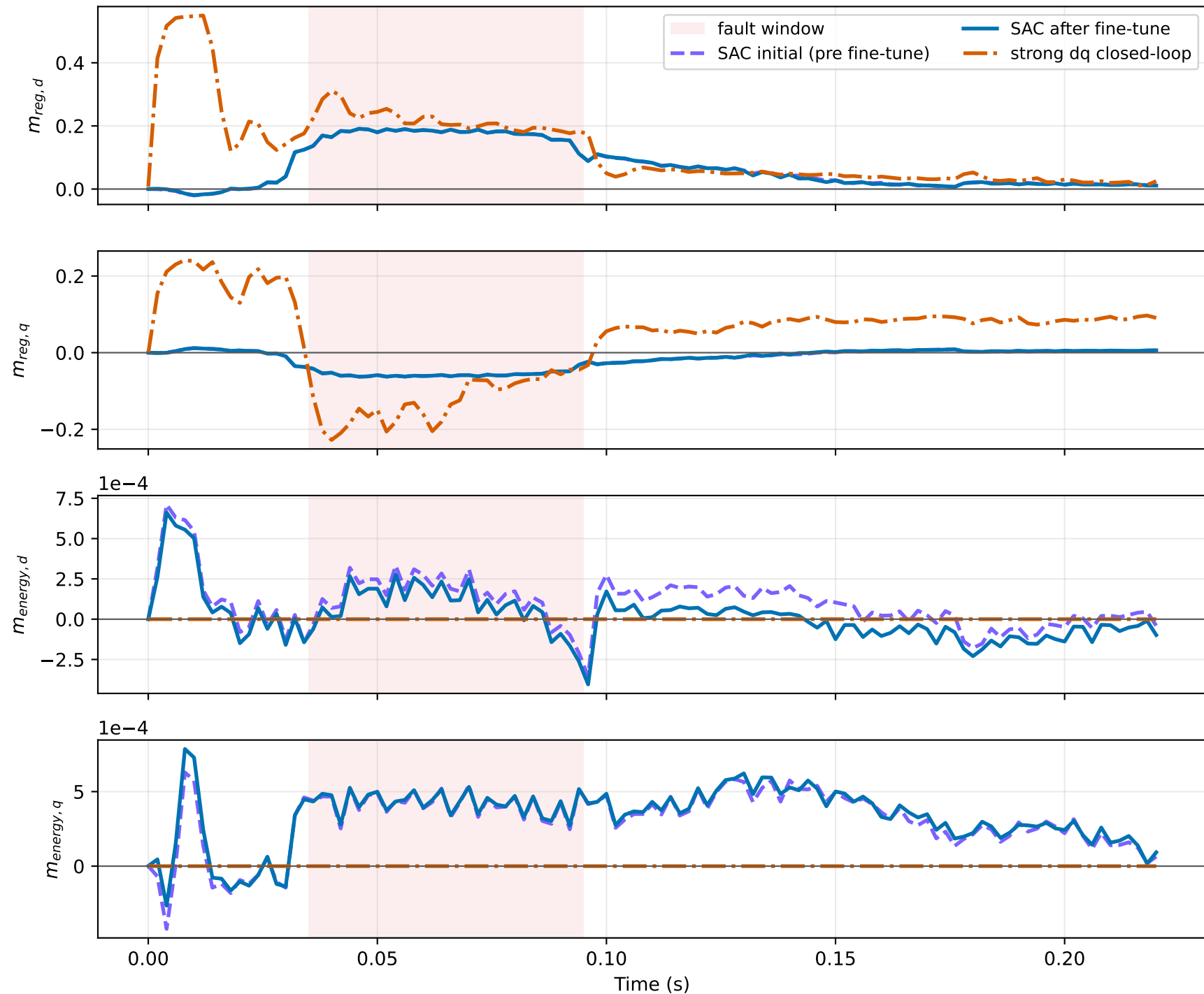
Controller modulation commands per 2-ms control step Topology2 balanced LVRT 0.90 pu / 60 ms
