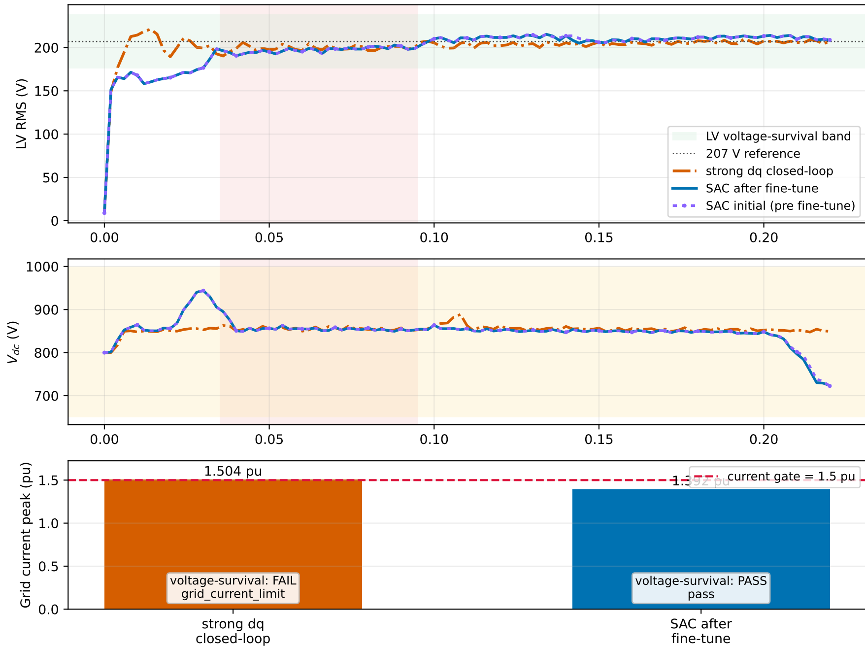
Voltage trace alone does not show the dq failure mechanism
