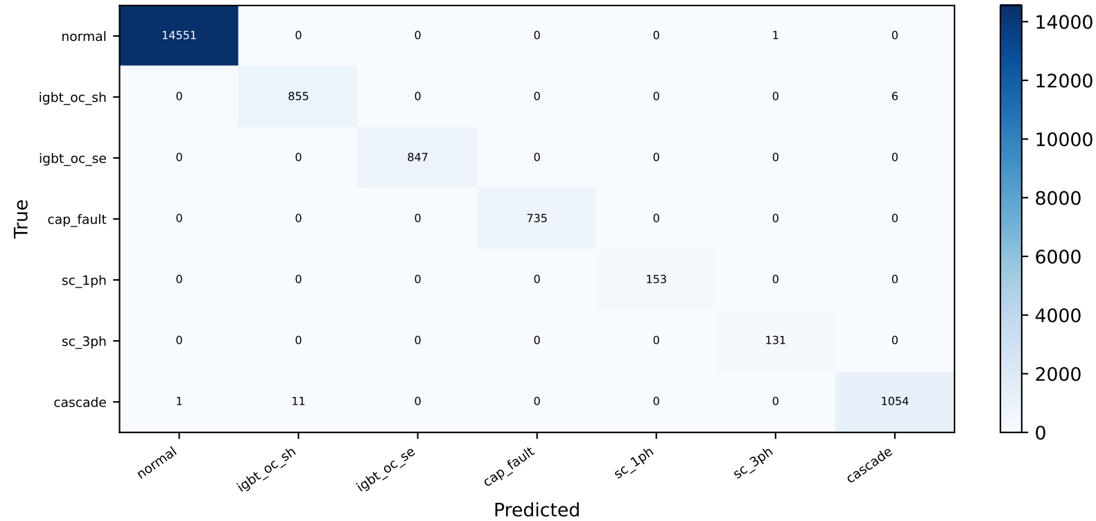
LSTM Confusion Matrix
