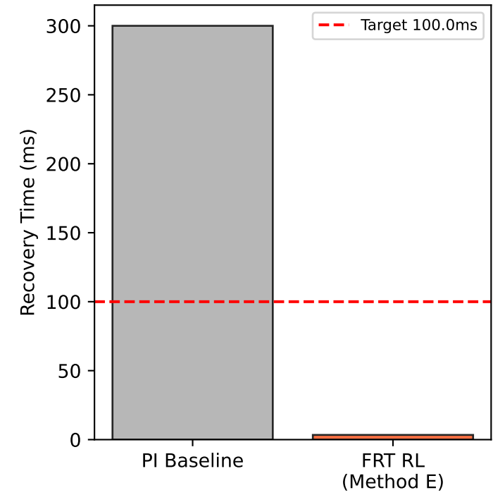
Post-Fault Recovery Time
