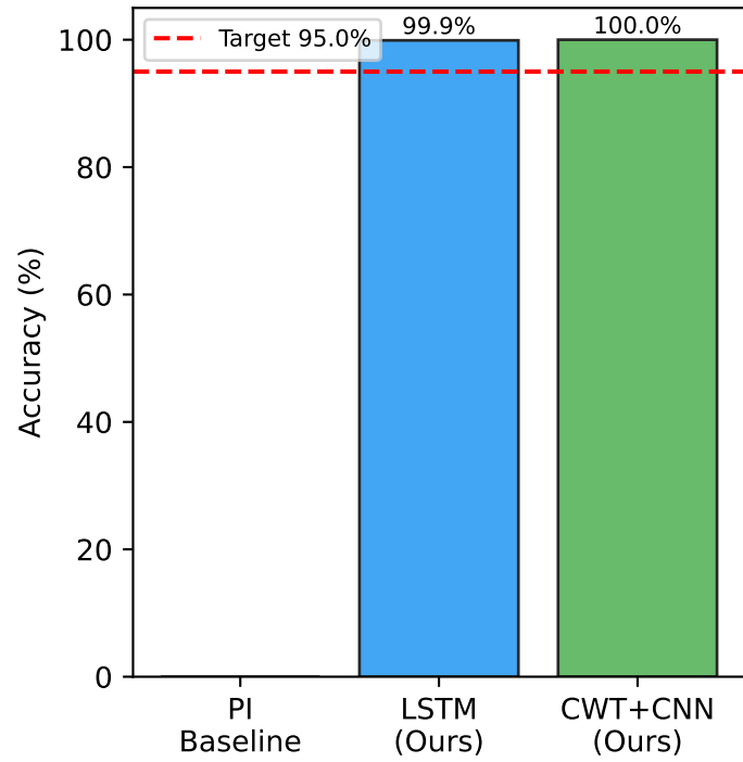
Fault Classification Accuracy
