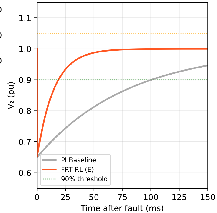
Voltage Recovery Comparison
