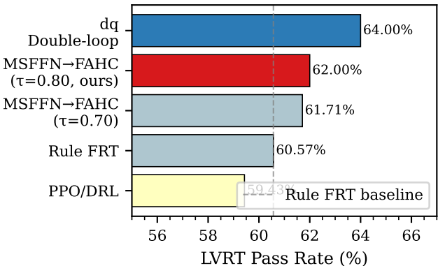
(c) LVRT Pass Rate — All Controllers
