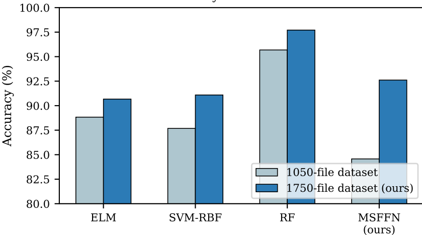
Accuracy vs. Dataset Size
