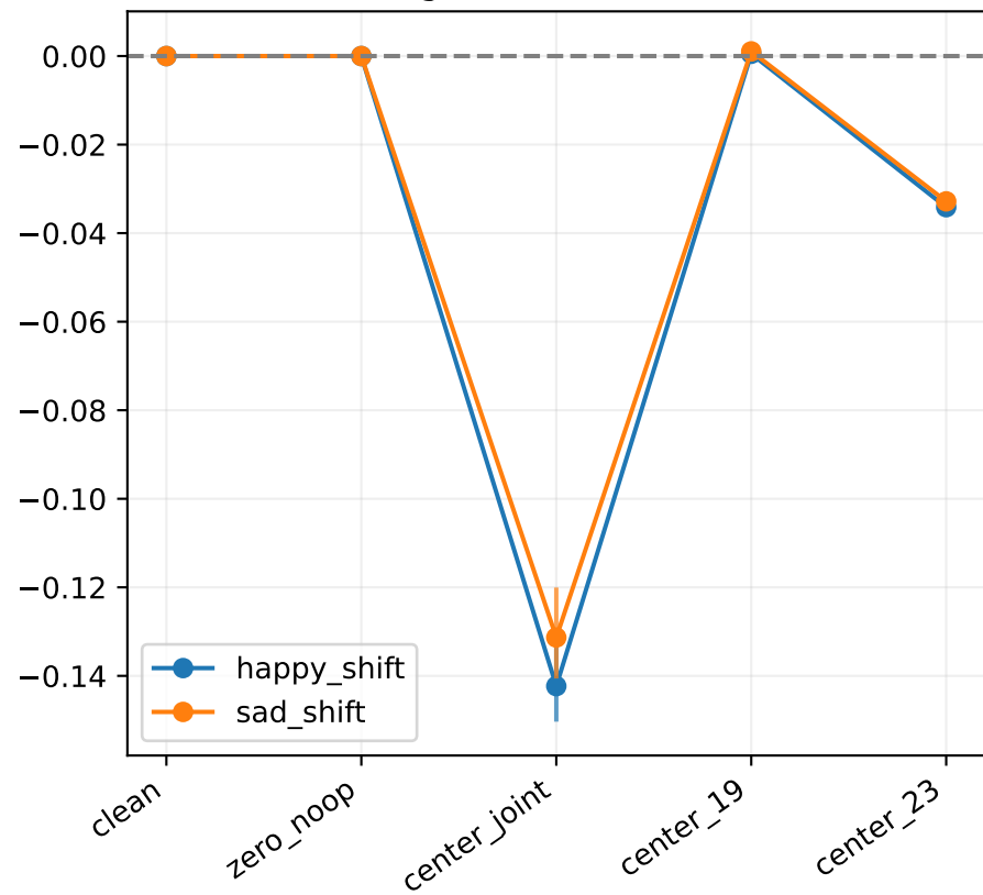
Margin shift from clean
