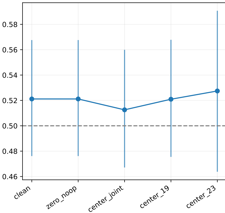
Model ROC-AUC
