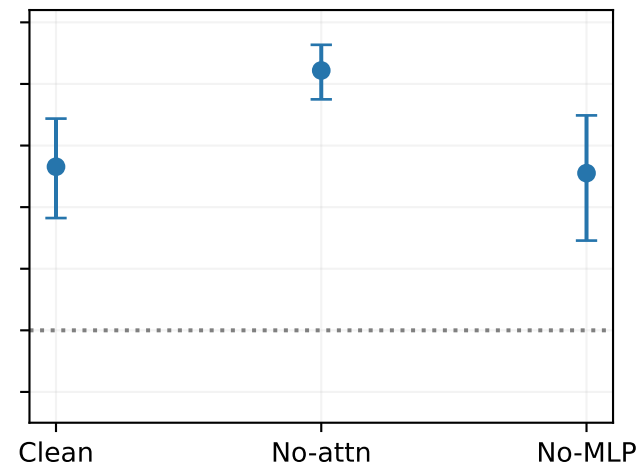
Both statements (macro)
