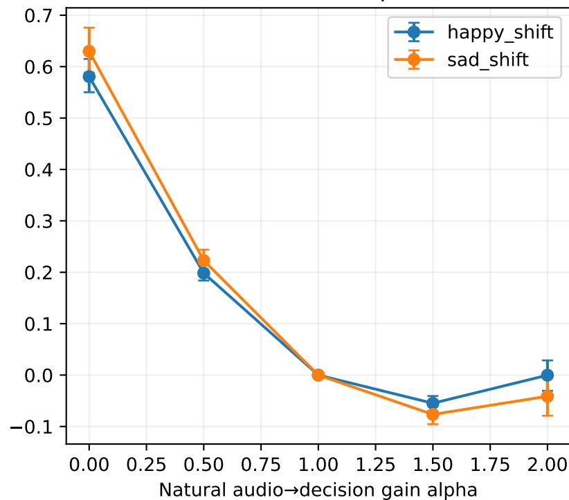
Shift relative to alpha=1
