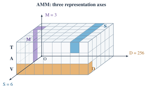
Figure 1: Tensor organization in AMM. Three aligned modality branches are expanded into S learned projection views with D hidden features. Colored cell groups highlight example vectors along the projection ( S ), modality ( M ), and hidden-feature ( D ) axes, with the other two indices fixed. The feature axis is drawn schematically. Learned views are not temporal steps.
