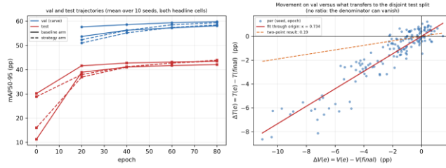
Fig. 4. Left: mean val and test trajectories over 10 seeds, both headline cells (baseline solid, strategy dashed). Right: per-(seed, epoch) val movement against what transfers to test — the ratio is not taken (its denominator can vanish); the fit through the origin is \kappa = 0.734 .
