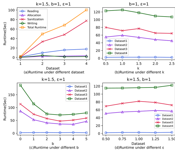
Fig. 6. Scalability analysis.
