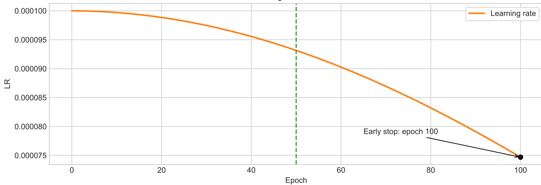
Learning Rate Schedule
