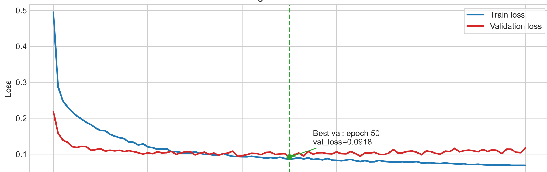
Generalization Gap
