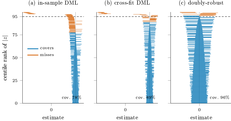
Figure 9: Zip plot of nominal 95% confidence-interval coverage [Morris et al., 2019] at the strong-effect, small-sample cell ( n = 500 , per- \sigma direct effect 0.10), 300 replications. Each horizontal segment is one replication’s interval, sorted bottom-to-top by the absolute z -statistic against the estimand (the estimator’s probability limit, gray vertical line); intervals that cover the estimand are blue and those that miss are orange, so the height at which the colour switches is the empirical coverage. The doubly-robust interval switches at the dashed nominal 95 line, the cross-fit DML interval close to it, and the in-sample DML influence-function interval well below it: its misses are too frequent and fan out symmetrically, the visual signature of an anticonservative variance rather than bias.
