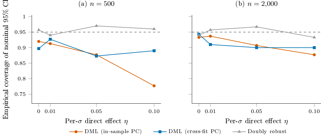
Figure 9: Finite-sample coverage of the nominal 95% influence-function interval for the embedding-valued treatment, across effect size \eta at n = 500 (a) and n = 2,000 (b), with 300 Monte Carlo replications per cell. The horizontal dashed line marks the nominal level. The in-sample principal-component DML interval, which treats the estimated leading component as a generated regressor, under-covers as the true effect grows, falling to 0.78 at n = 500 , because the orthogonal-score variance does not capture the sampling variability of the estimated treatment direction. Forming the component out of fold (cross-fit PC) recovers most of the lost coverage, and the doubly-robust estimator, which does not estimate a continuous direction, is calibrated throughout but has no power against the graded effect.
