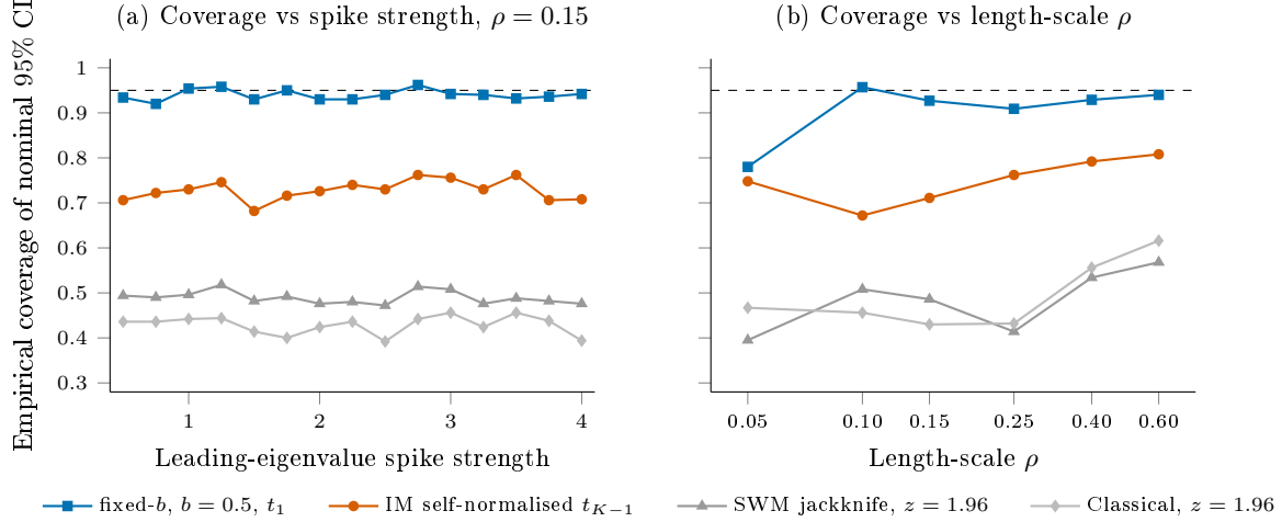
Figure 10: Empirical coverage of nominal 95% confidence intervals across the Davis–Kahan stress simulation, with 1,000 Monte Carlo replications per cell. The horizontal dashed line in each panel marks the nominal level. Panel (a) varies the leading-eigenvalue spike strength while holding the spatial length-scale at \rho = 0.15 , and panel (b) varies the length-scale on a log axis while holding the spike strength at its central value. The Salerno–Wu–McCormick jackknife paired with the conventional z = 1.96 critical value sits near 0.49 across both axes, the Ibragimov–Müller self-normalised t_{K-1} paired with the same fold-mean variance sits near 0.73, and the fixed- b envelope of Sun et al. [2008] at b = 0.5 reaches roughly 0.93 at the cost of substantially wider intervals. The seven remaining inference rules reported in Table 13 bunch within the band traced by classical and SWM-with- z and are omitted from the figure for legibility.
