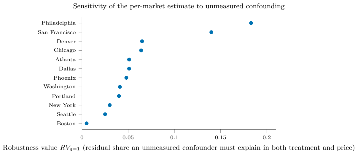
Figure 10: Robustness value for each market’s sentence-BERT estimate, the share of residual variance an unmeasured confounder would need to explain in both the treatment and log price to drive the estimate to zero, following Cinelli and Hazlett [2020]. Larger values are more robust. The estimate is most robust in Philadelphia (0.18) and San Francisco (0.14) and most fragile in the markets whose point estimates are already near zero. The modest robustness values in several markets are the reason we read the per-market estimates as associational and sensitivity-bounded rather than causal.
