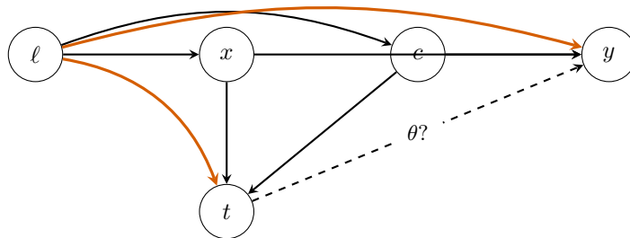
Figure 1: The structure the paper adjudicates. Location \ell is exogenous and feeds the property attributes x , the contextual features c , the listing text t , and the price y . The two highlighted edges \ell \rightarrow t and \ell \rightarrow y form the spatial-confounding backdoor, the reason text and price are associated in part simply because both depend on where the property sits. The dashed edge labelled \theta is the direct effect of text on price, the quantity we estimate, and the empirical question is how much of the text-price association is that direct edge rather than the backdoor through \ell . Conditioning on \{\ell, x, c\} blocks the backdoor and identifies \theta ; whether \theta is zero or positive is what the twelve markets decide.
