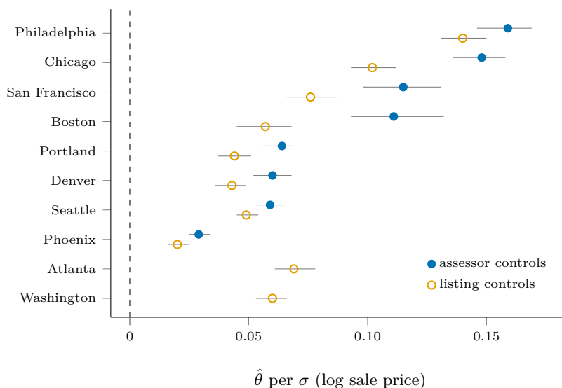
Figure 11: Per-market effect of the leading listing-text direction on log realized sale price, oriented so the effect is positive. Filled blue markers use exogenous county-assessor structural controls (the primary, controlled-direct-effect specification); open amber markers use agent-reported listing attributes (the bad-control sensitivity bound). Gray whiskers are 95% tract cluster-bootstrap intervals ( B = 300 ); the dashed line marks the null. Washington and Atlanta lack a county structural source and carry only the listing specification. The listing effect lies inside the assessor effect in every market where both are estimated, the signature of controlling for text-entangled attributes. Numerical values appear in Table 15.
