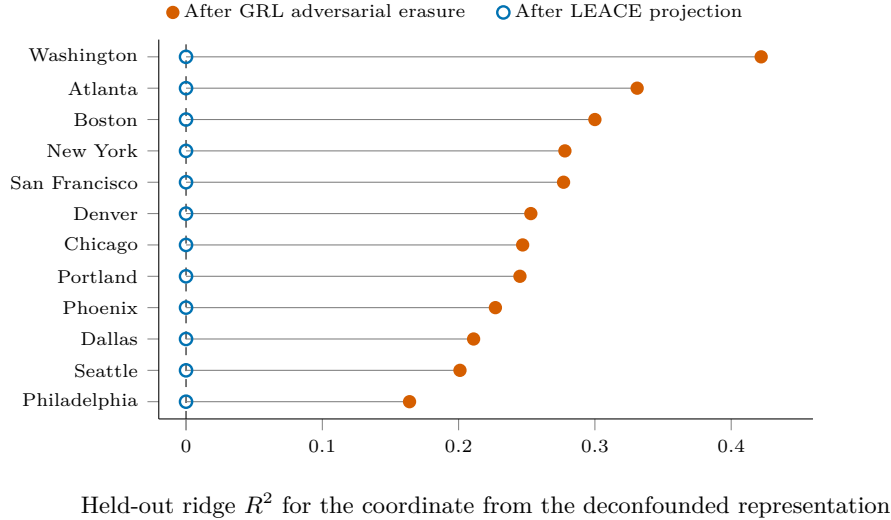
Figure 4: The frozen-probe diagnostic applied to two erasure methods, in each of the twelve markets. A ridge probe of the latitude-longitude coordinate is trained from scratch on the deconfounded representation. Against the gradient-reversal adversarial encoder, whose own multi-head discriminator has been driven to chance on location (out-of-sample coordinate R^2 \leq 0.07 across the panel), the fresh probe still recovers the coordinate at R^2 between 0.16 and 0.42; against the LEACE projection the same probe sits at the chance baseline, the exact-guardedness property of closed-form erasure. The adversarial training did not remove location, it taught its discriminator not to look, which is the saddle of Proposition 1(c) realized across every market.
