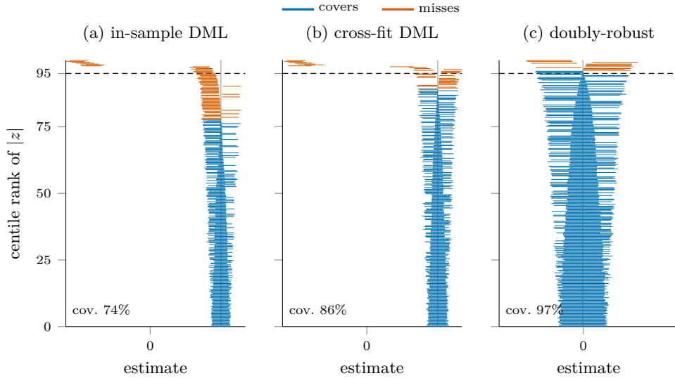
Figure 5: Zip plot of nominal 95% confidence-interval coverage [Morris et al., 2019] at the strong-effect, small-sample cell ( n = 500 , per- \sigma direct effect 0.10), 300 replications. Each horizontal segment is one replication’s interval, sorted bottom-to-top by the absolute z -statistic against the estimand (the estimator’s probability limit, gray vertical line); intervals that cover the estimand are blue and those that miss are orange, so the height at which the color switches is the empirical coverage. The doubly-robust interval switches at the dashed nominal 95 line, the cross-fit DML interval close to it, and the in-sample DML influence-function interval well below it: its misses are too frequent and fan out symmetrically, the visual signature of an anticonservative variance rather than bias.
