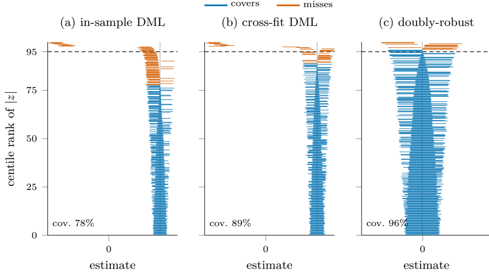
Figure 10: Zip plot of nominal 95% confidence-interval coverage [Morris et al., 2019] at the strong-effect, small-sample cell ( n = 500 , per- \sigma direct effect 0.10), 300 replications. Each horizontal segment is one replication’s interval, sorted bottom-to-top by the absolute z -statistic against the estimand (the estimator’s probability limit, gray vertical line); intervals that cover the estimand are blue and those that miss are orange, so the height at which the colour switches is the empirical coverage. The doubly-robust interval switches at the dashed nominal 95 line, the cross-fit DML interval close to it, and the in-sample DML influence-function interval well below it: its misses are too frequent and fan out symmetrically, the visual signature of an anticonservative variance rather than bias.
