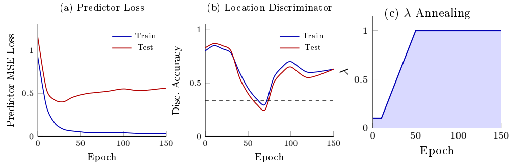
Figure 8: Adversarial training dynamics for San Francisco. (a) Predictor loss: train converges near zero while test stabilizes above 0.5. (b) Discriminator accuracy drops toward the dashed random baseline of 1/3 as \lambda ramps, then partially recovers. (c) The \lambda annealing schedule ramps from 0.1 to 1.0 over epochs 10–50.
