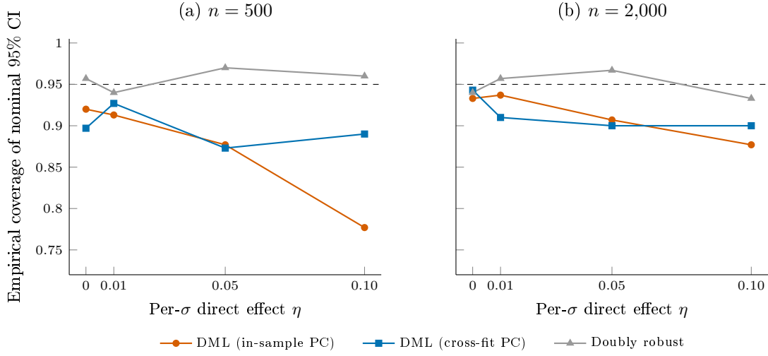
Figure 2: Finite-sample coverage of the nominal 95% influence-function interval for the embedding-valued treatment, across effect size \eta at n = 500 (a) and n = 2,000 (b), with 300 Monte Carlo replications per cell. The horizontal dashed line marks the nominal level. The in-sample principal-component DML interval, which treats the estimated leading component as a generated regressor, under-covers as the true effect grows, falling to 0.78 at n = 500 , because the orthogonal-score variance does not capture the sampling variability of the estimated treatment direction. Forming the component out of fold (cross-fit PC) recovers most of the lost coverage, and the doubly-robust estimator, which does not estimate a continuous direction, is calibrated throughout but has no power against the graded effect.
