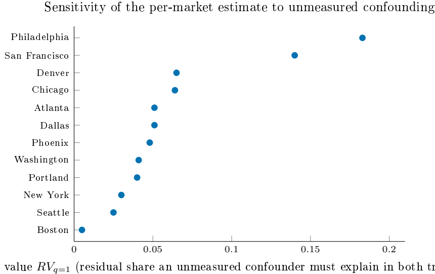
Figure 5: Robustness value for each market’s sentence-BERT effect, the share of residual variance an unmeasured confounder would need to explain in both the treatment and log price to drive the estimate to zero, following Cinelli and Hazlett [2020]. Larger values are more robust. The estimate is most robust in Philadelphia (0.18) and San Francisco (0.14) and most fragile in the markets whose point estimates are already near zero. The modest robustness values in several markets are the reason we read the per-market estimates as associational and sensitivity-bounded rather than cleanly causal.
