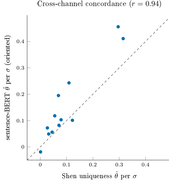
Figure 6: Per-market estimates of the two embedding channels against each other, with the 45° identity line. The two channels co-move almost perfectly across markets (Pearson r = 0.94 ), so they recover one underlying signal under two encodings rather than two independent measurements; the systematic departure from the identity line reflects that the sentence-BERT axis is roughly twice the Shen channel in magnitude, not a difference in which markets carry the signal.
