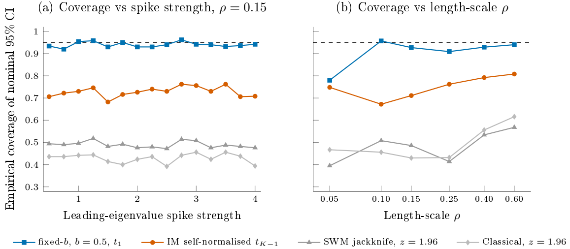
Figure 8: Empirical coverage of nominal 95% confidence intervals across the Davis–Kahan stress simulation, with 1,000 Monte Carlo replications per cell. The horizontal dashed line in each panel marks the nominal level. Panel (a) varies the leading-eigenvalue spike strength while holding the spatial length-scale at \rho = 0.15 , and panel (b) varies the length-scale on a log axis while holding the spike strength at its central value. The Salerno–Wu–McCormick jackknife paired with the conventional z = 1.96 critical value sits near 0.49 across both axes, the Ibragimov–Müller self-normalised t_{K-1} paired with the same fold-mean variance sits near 0.73, and the fixed- b envelope of Sun et al. [2008] at b = 0.5 reaches roughly 0.93 at the cost of substantially wider intervals. The seven remaining inference rules reported in Table 13 bunch within the band traced by classical and SWM-with- z and are omitted from the figure for legibility.
