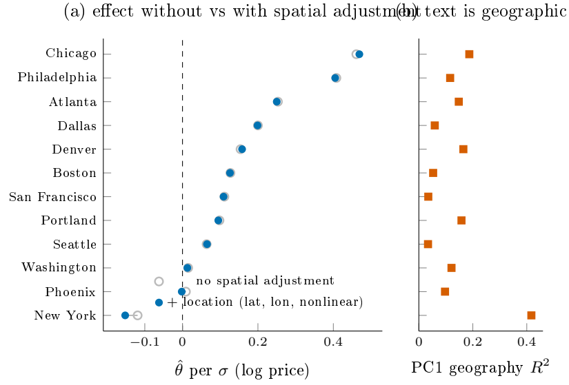
Figure 7: Is the per-market text-price effect spatially confounded? Holding the leading text principal component fixed as the treatment, panel (a) plots its DML effect on log price controlling for the structured confounders without (open) and with (filled) a location adjustment that adds latitude, longitude, and their quadratic and interaction terms to the confounder set. The two estimates nearly coincide in eleven of twelve markets, with a confounded share below five percent of the effect; New York is the exception, where the location adjustment moves the estimate by about a quarter of its magnitude without changing its sign. Panel (b) reports the share of the treatment’s own variance that the location basis explains, which reaches 0.42 in New York and exceeds 0.10 in six markets, so the robustness in panel (a) is not an artifact of a treatment that carries no geography: the text direction does encode location, yet that location component does not drive its price effect.
