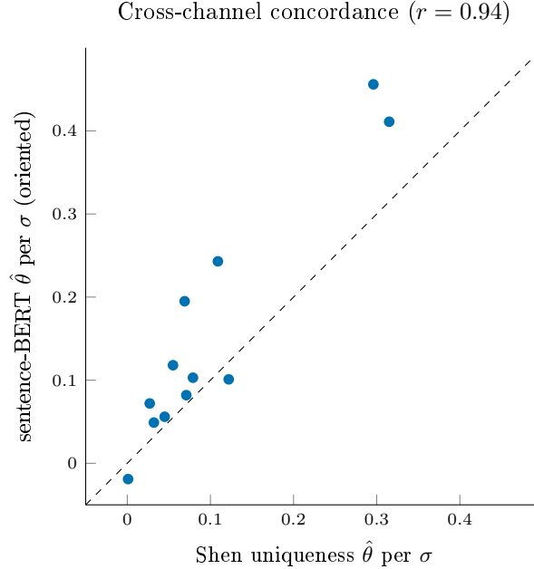
Figure 7: Per-market estimates of the two embedding channels against each other, with the 45^\circ identity line. The two channels co-move almost perfectly across markets (Pearson r = 0.94 ), so they recover one underlying signal under two encodings rather than two independent measurements; the systematic departure from the identity line reflects that the sentence-BERT axis is roughly twice the Shen channel in magnitude, not a difference in which markets carry the signal.
