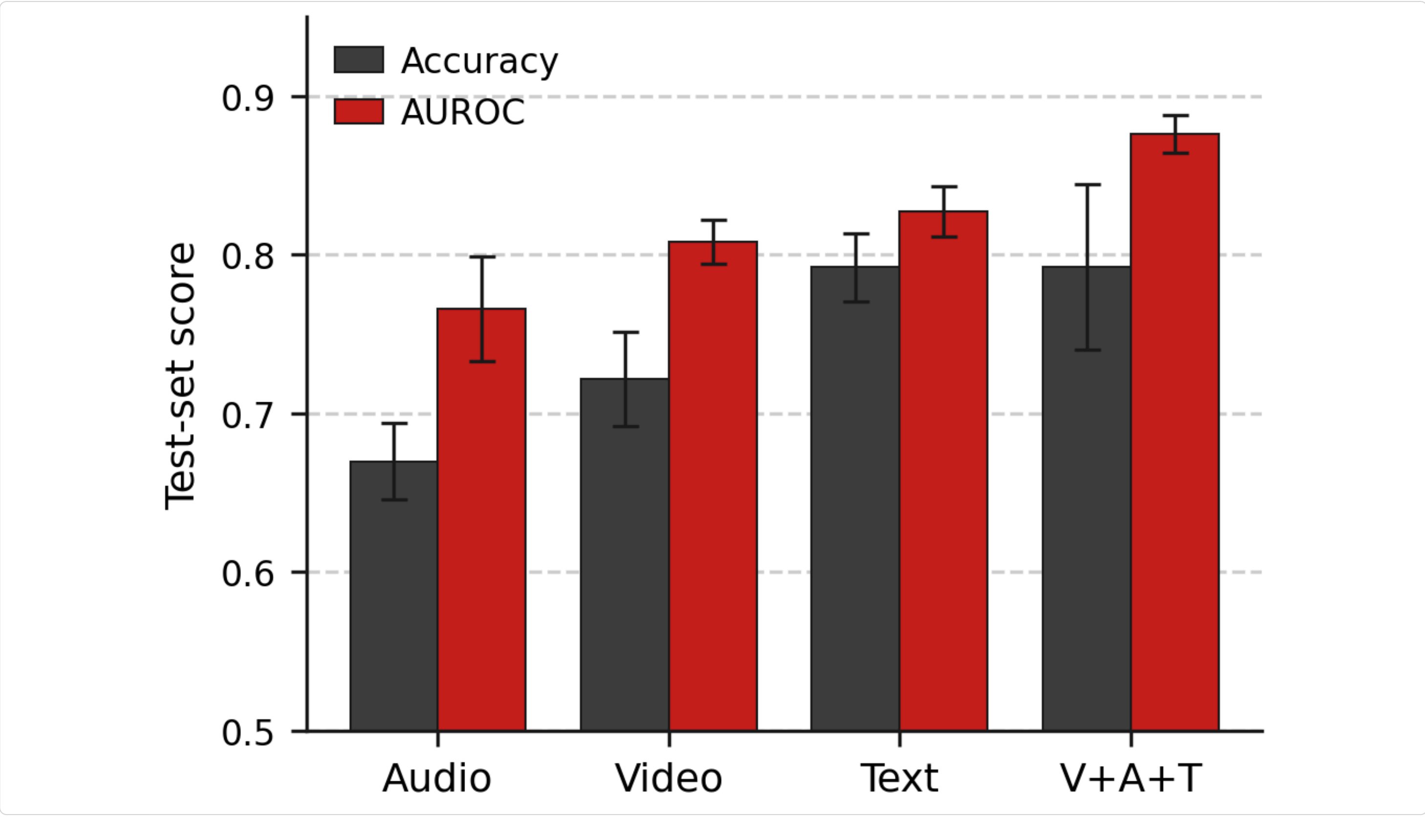
Figure 1. Test accuracy and AUROC across the four models, mean ± std over 3 seeds, sorted ascending by AUROC.
