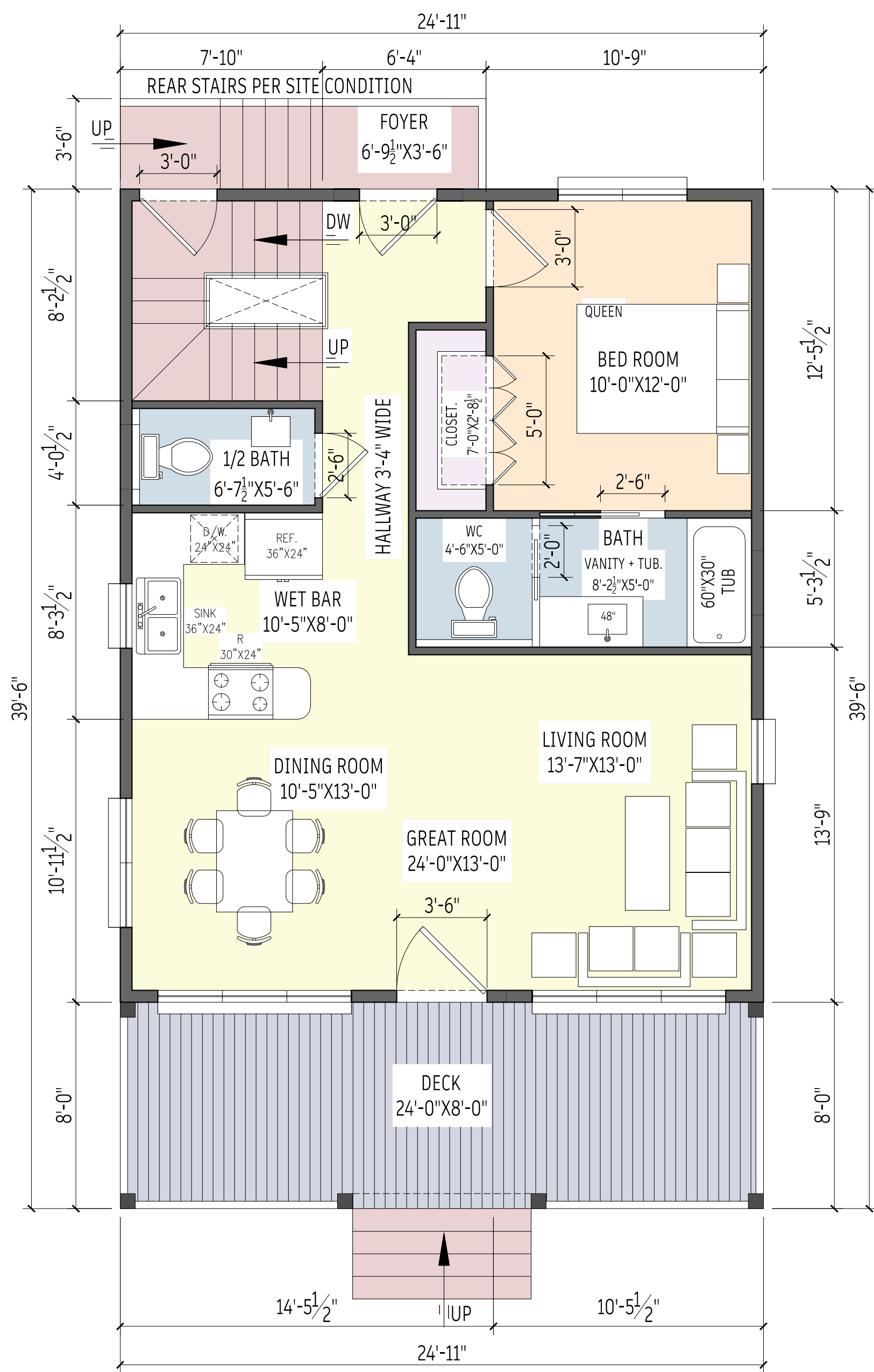
2 FIRST FLOOR PLAN. Scale: 1/4" = 1'.0"
