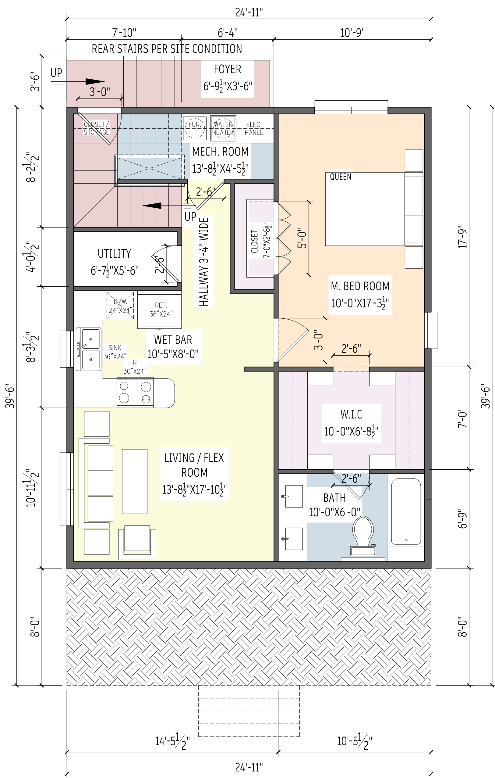
1 BASEMENT FLOOR PLAN. Scale: 1/4" = 1'.0"
