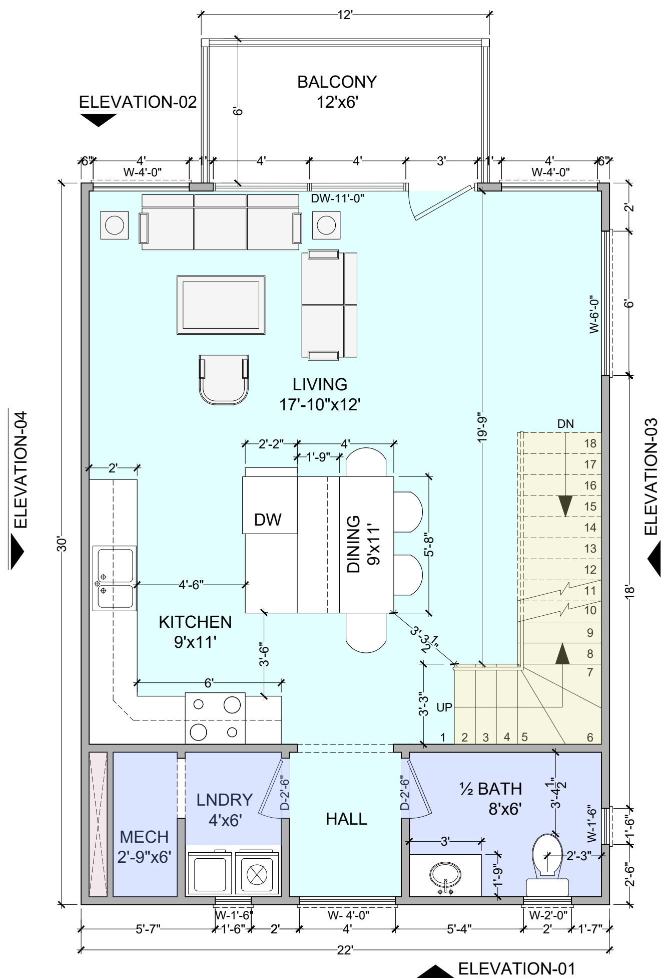
SECOND FLOOR PLAN SCALE: 1/4" = 1'-0"
