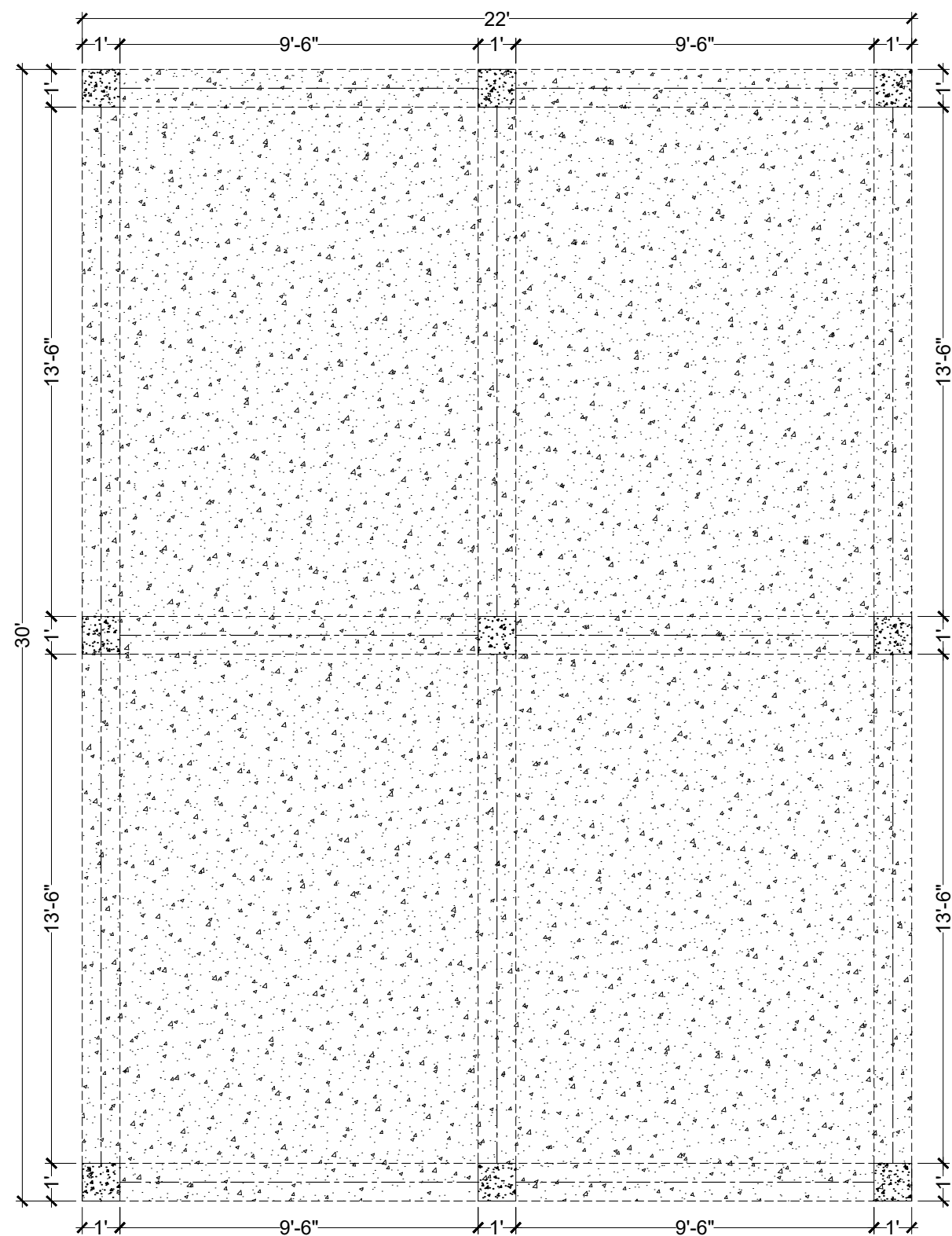
SLAB FOUNDATION PLAN SCALE: 1/4" = 1'-0"
