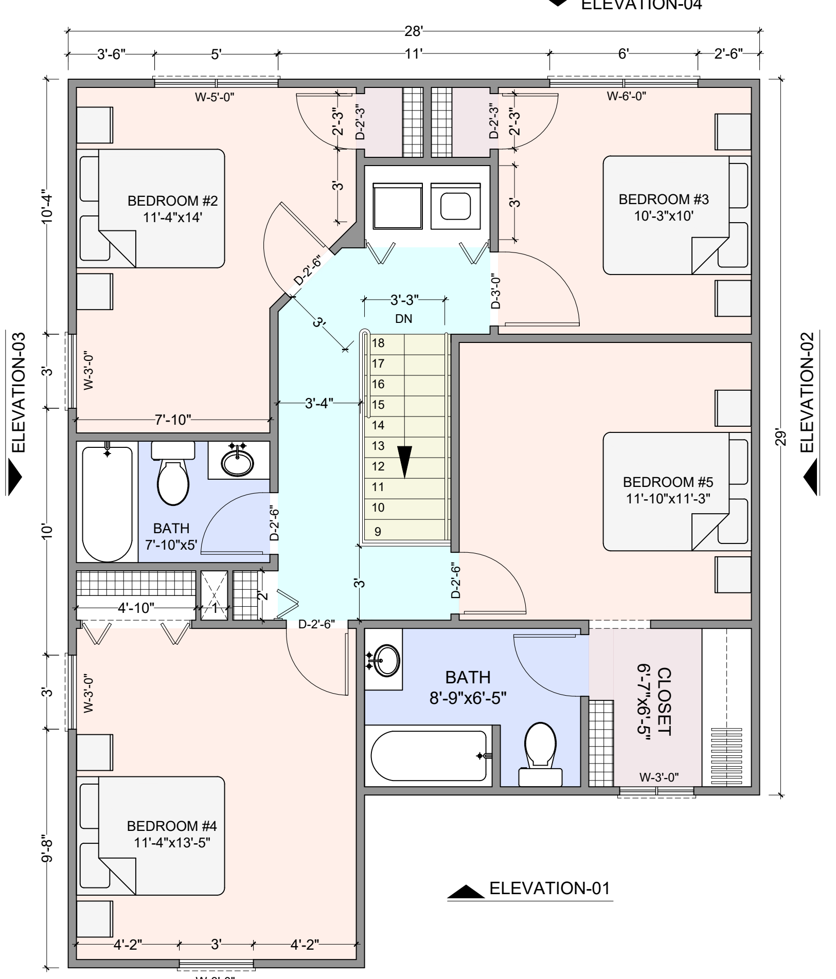
SECOND FLOOR PLAN SCALE: 1/4" = 1'-0"
