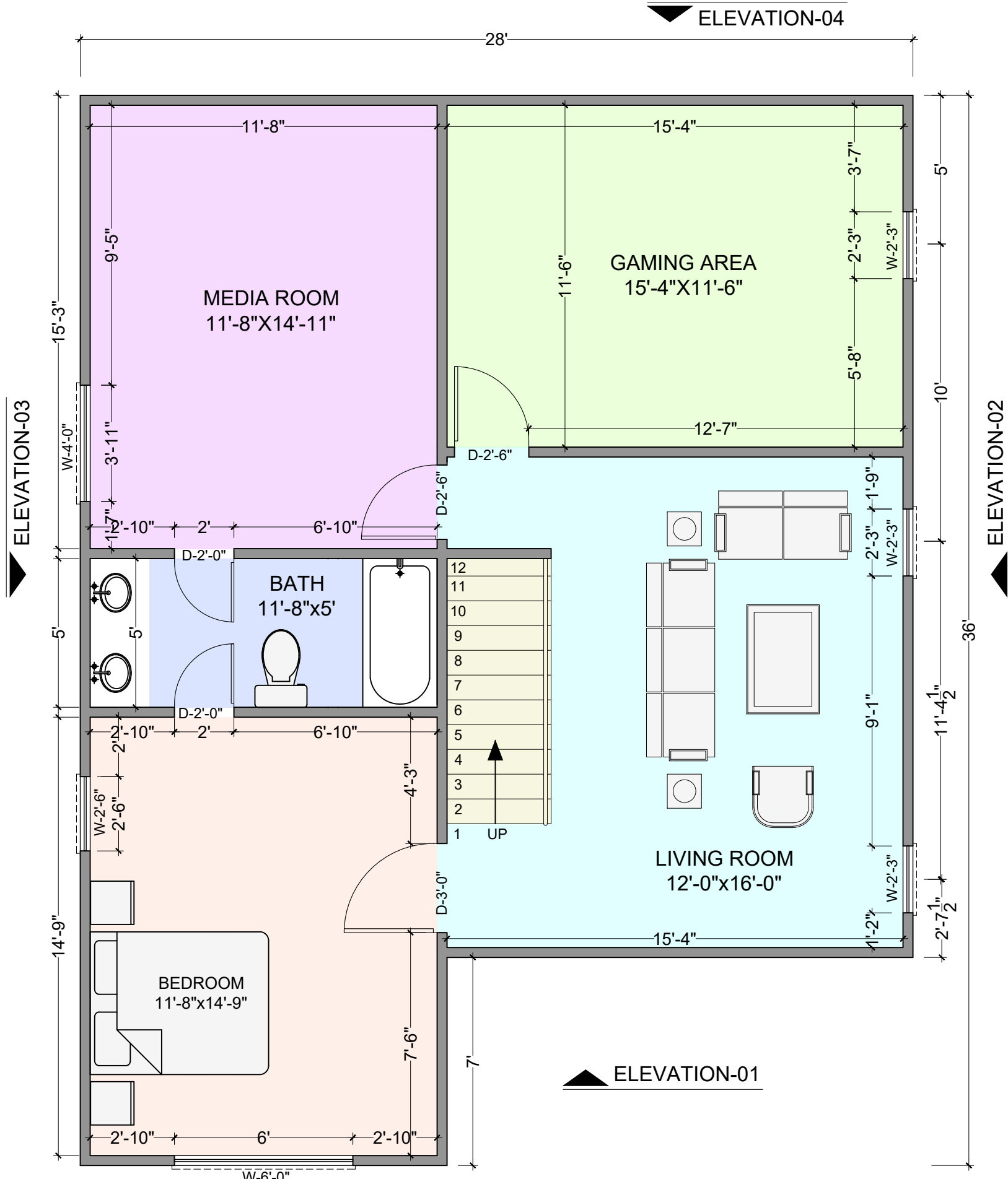
BASEMENT FLOOR PLAN SCALE: 1/4" = 1'-0"
