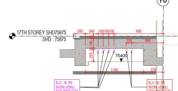
6 Recess Beam -Sec 06 1 : 25
