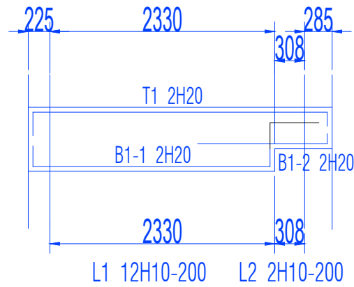
38 # RS-HB34 200x665/430 TOB: 0
