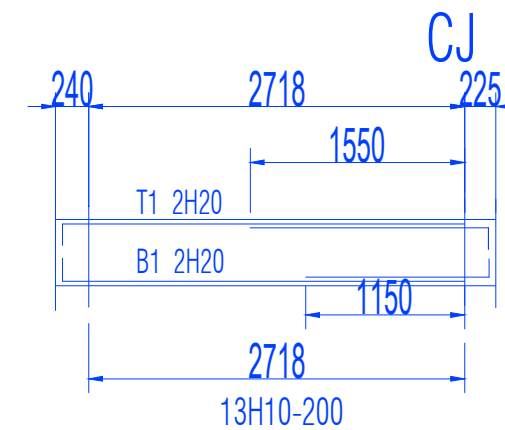
43 # RS-HB40 200x480 TOB: +10
