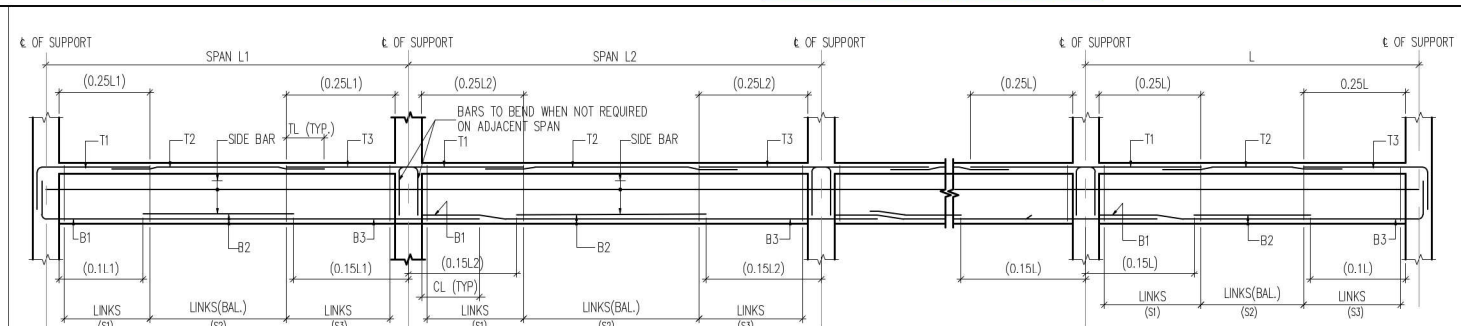
LEFT END SPAN TYPICAL INTERMEDIATE SPAN TYPICAL INTERMEDIATE SPAN RIGHT END SPAN TYPICAL CONTINUOUS SPAN BEAM
