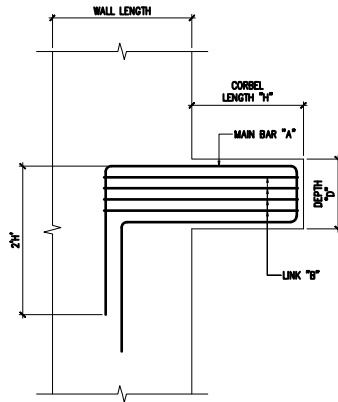
DETAIL A - STANDARD CORBEL DETAIL
