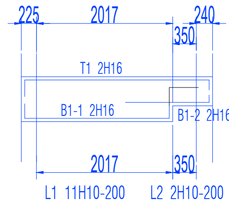
42 # RS-HB39 200x665/430 TOB: 0
