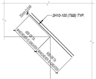
TYPICAL TRIMMER BARS AT RE-ENTRANT CORNER
