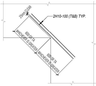
TYPICAL TRIMMER BARS AT RE-ENTRANT CORNER SCALE: 1:25
