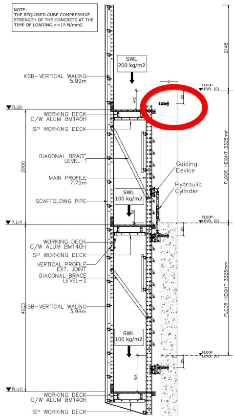
NUFORM CLIMBING SCAFFOLD SYSTEM TYPICAL SECTION DETAIL FOR WALL 240mm
