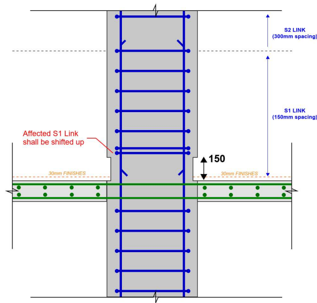
RESI RC COLUMN SKIRTING RECESS DETAIL
