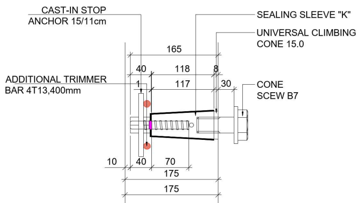
SET UP FOR UNIVERSAL CLIMBING CONE 15.0 WITH STOP ANCHOR 15/11 cm (WALL THICKNESS >=175~200mm)
