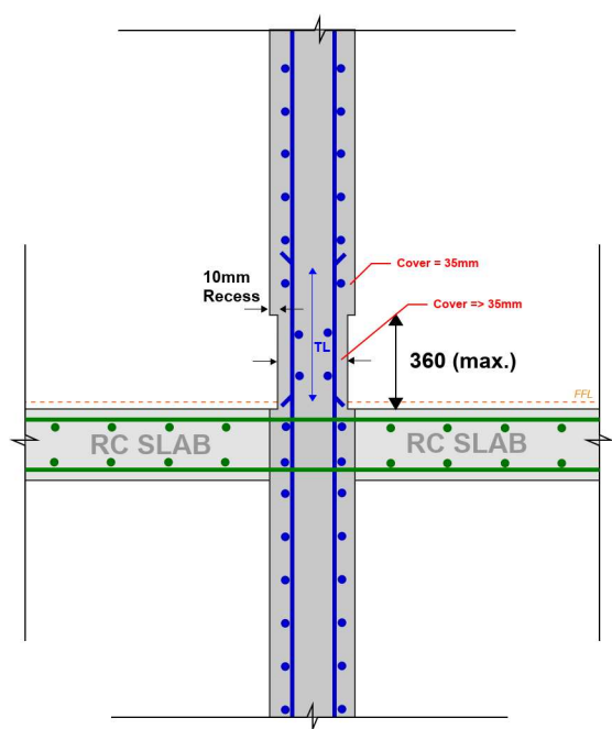
RESI RC WALL SKIRTING RECESS DETAIL
