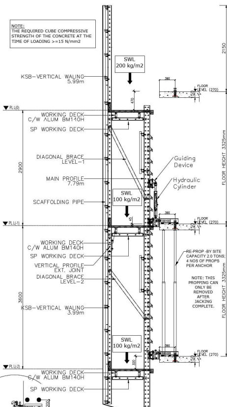
NUFORM PERIMETER SCAFFOLD SYSTEM TYPICAL SECTION DETAIL FOR CAST IN-SITU RC LEDGE 150mm
