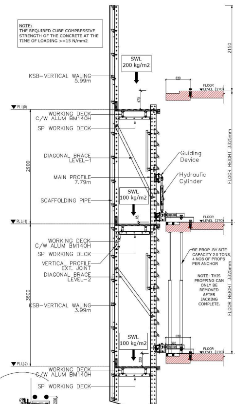
NUFORM PERIMETER SCAFFOLD SYSTEM TYPICAL SECTION DETAIL FOR CAST IN-SITU BALCONY 180mm
