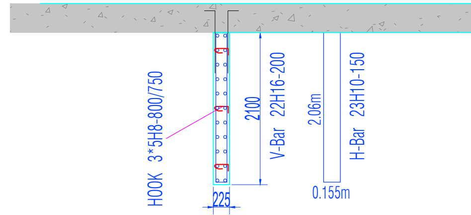
35TW33-1 225x2100 TL = 52D
